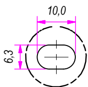
B (1:1)
