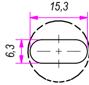
C (1:1)
