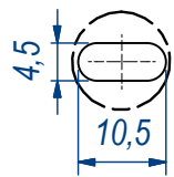
B (1:1) C (1:1)
