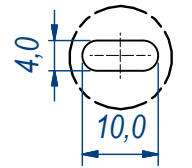
D (1:1)
